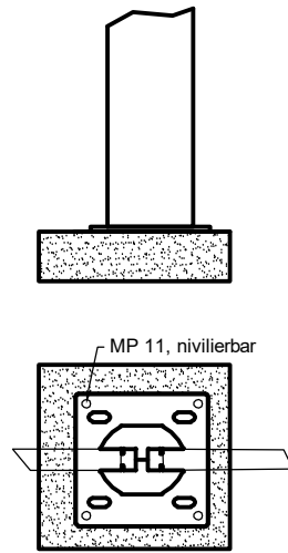
Standardmontage
