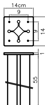
Fundament: Aluminiumsockel
